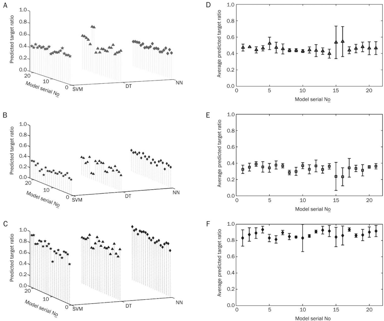
Figure 6. Evaluation of the 21 parallel models against three testing datasets. Evaluation against (A) Dataset I, clinical phase II targets (size: 202), (B) Dataset II, human proteome (size: 20 025), and (C) Dataset III, targets of withdrawn drugs (size: 55). Mean values and standard errors of the 21 models using the 3 algorithms against (D) Dataset I, (E) Dataset II, and (F) Dataset III.
