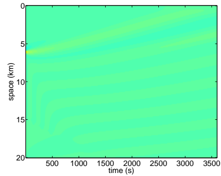
(h) M = 3, \gamma_2 = 0.1, c \neq 0
