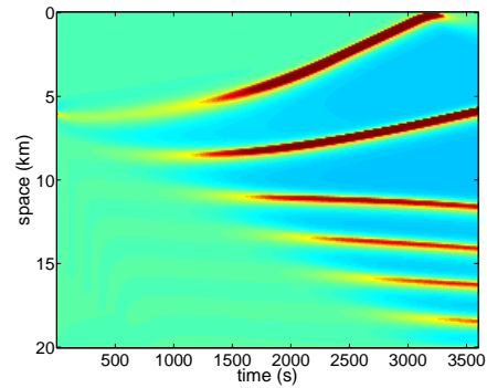
(f) M = 3, \gamma_2 = 0.2, c \neq 0
