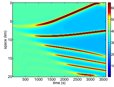
(b) M = 1, \gamma_2 = 0.2, c = 0
