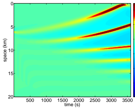
(g) M = 1, \gamma_2 = 0.1, c \neq 0
