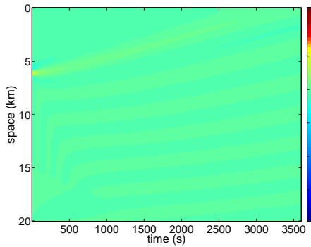
(e) M = 3, \gamma_2 = 0, c \neq 0
