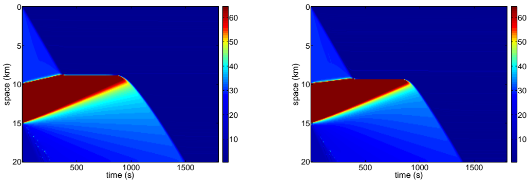
(a) M = 3, \gamma_2 = 0, c \neq 0
