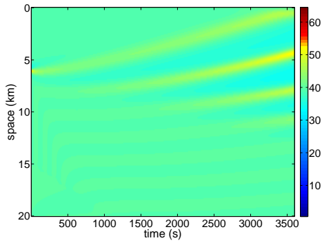
(a) M = 1, \gamma_2 = 0, c = 0
