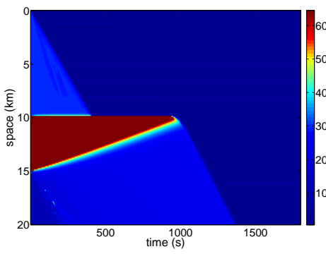
(c) M = 3, \gamma_2 = 0.5, c \neq 0
