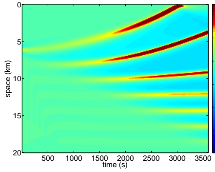
(c) M = 1, \gamma_2 = 0, c \neq 0
