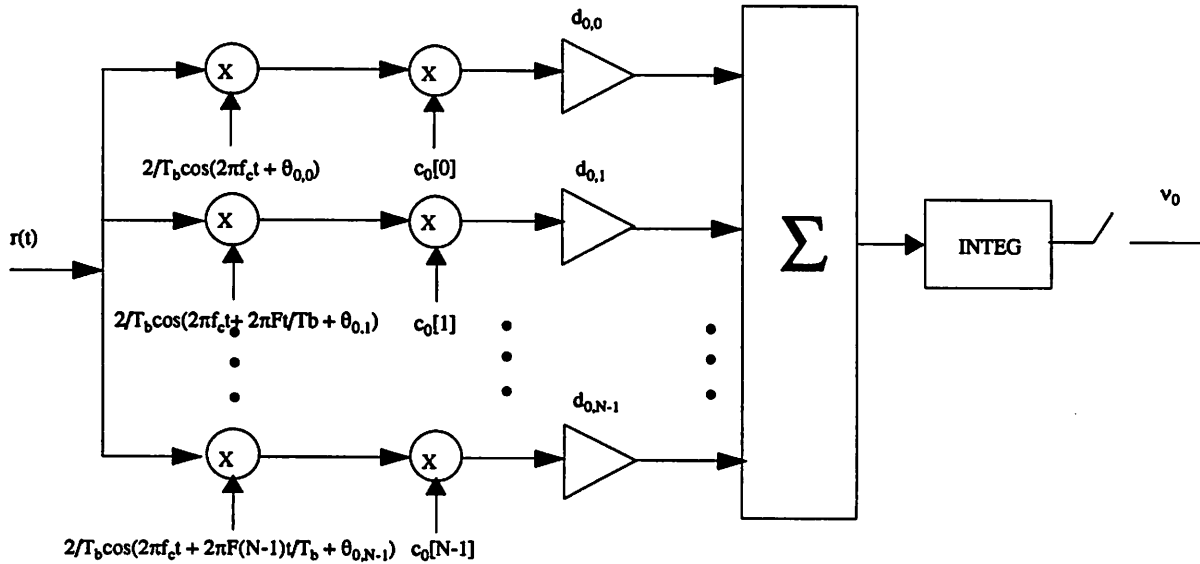
Fig. 3 Receiver Model
