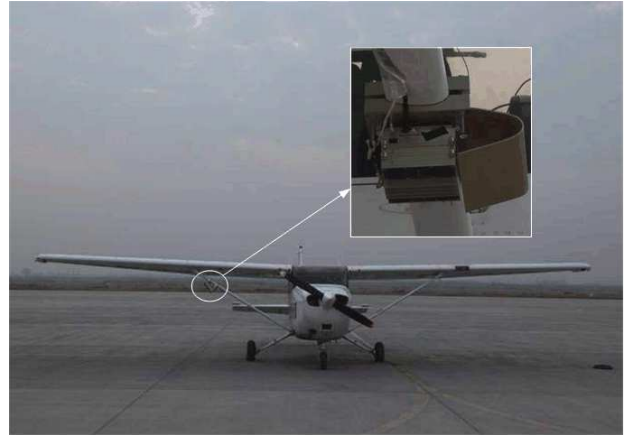
Fig. 9. Photograph of the airborne platform and the sensor.
