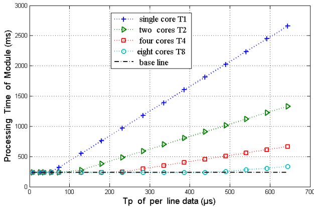
Fig. 8. Time consumption of parallel model.
