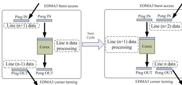
Fig. 5. Single core PingPong processing flow.
