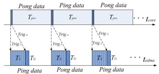
Fig. 6. Time sequence of single core processing.
