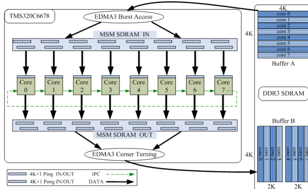
Fig. 4. Block diagram of parallel processing.
