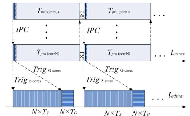
Fig. 7. Time sequence of N cores parallel processing.
