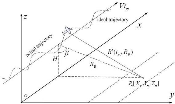
Fig. 1. Imaging geometry of airborne test.
