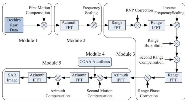
Fig. 2. Processing flow of FSA and its modularization.
