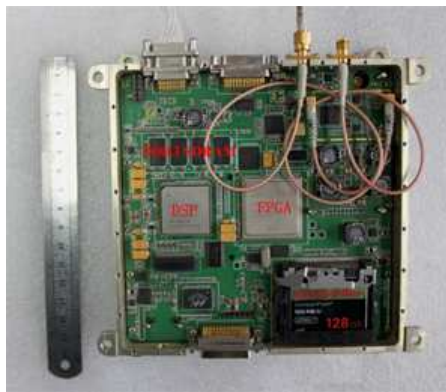
Fig. 3. The FMCW SAR processing board.
