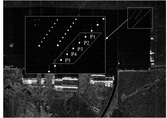
Fig. 11. Real-time processing result with corner reflectors.
