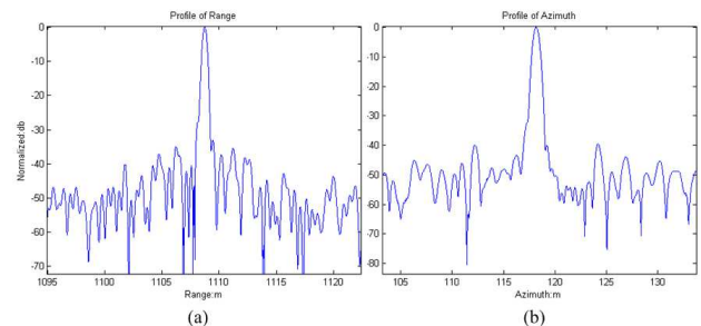
Fig. 12. Profiles of P2 in (a) range and (b) azimuth.
