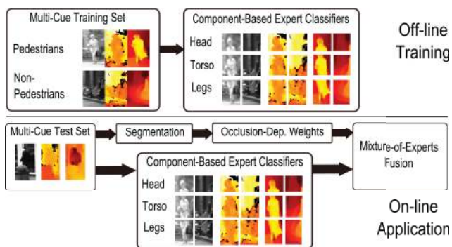
Figure 1. Framework overview. Multi-cue component-based expert classifiers are trained off-line on features derived from intensity, depth and motion. On-line, multi-cue segmentation is applied to determine occlusion-dependent component weights for expert fusion. Data samples are shown in terms of intensity images, dense depth maps and dense optical flow (left to right).
