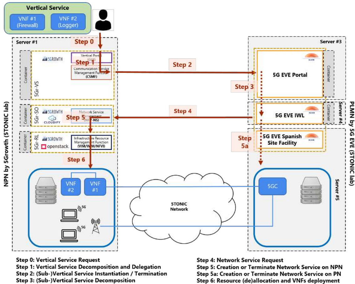
FIGURE 6. Evaluation scenario of PoC #1 Comprising the Integration of 5Growth and 5G EVE Platforms (SNPN with RAN sharing deployment)
