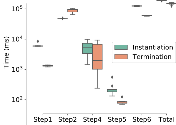
FIGURE 8. Service Instantiation and Termination Time Profiling (PoC #1)
