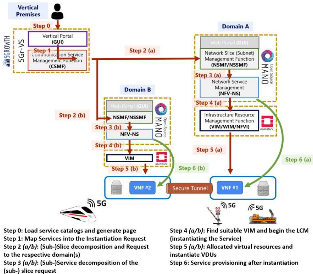
FIGURE 10. Evaluation Scenario of PoC #2 Comprising the Integration of 5Growth platform and Two OSM-based Domains (PNI-NPN with full sharing deployment)
