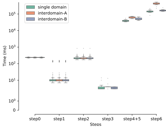
FIGURE 11. Instantiation Time Profiling of the E2E Vertical Slice (PoC #2)
