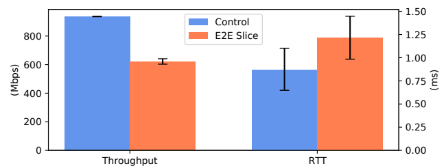
FIGURE 12. Impact on E2E Communication (PoC #2) (average values with 95% confidence interval)
