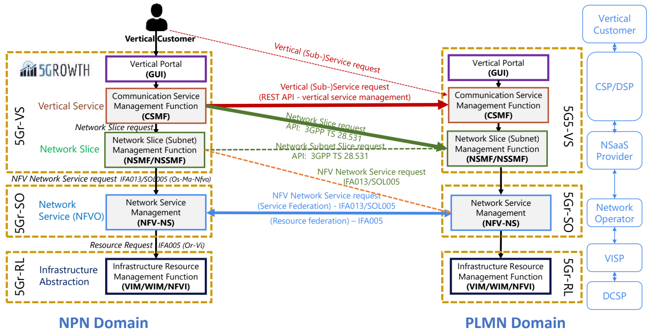
FIGURE 2. Multi-Domain options for NPN and PLMN Integration (PNI-NPN)
