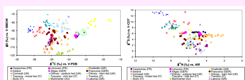
Figures 2 and 3: Carbon vs. hydrogen and nitrogen vs. sulfur isotopic ratios of lamb meat defatted dry mass (protein)
