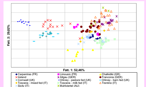
Figure 4: Plot of the first two principal components
