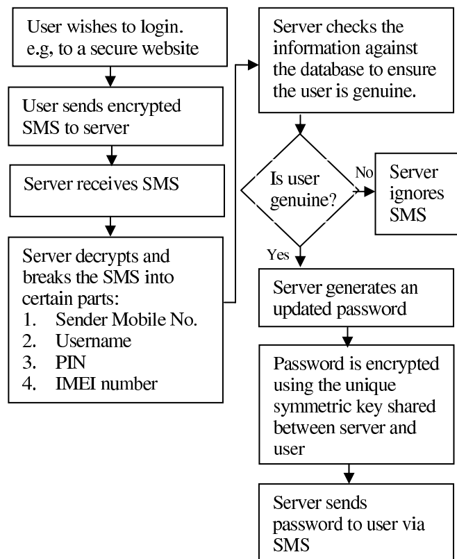
Figure 1: The connection-less process of generating the OTP.
