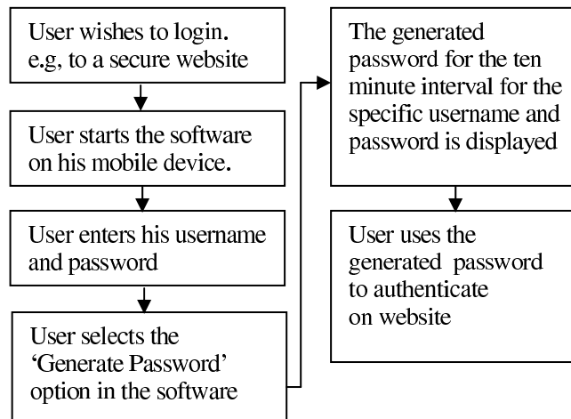
Figure 1: The connection-less process of generating the OTP.
