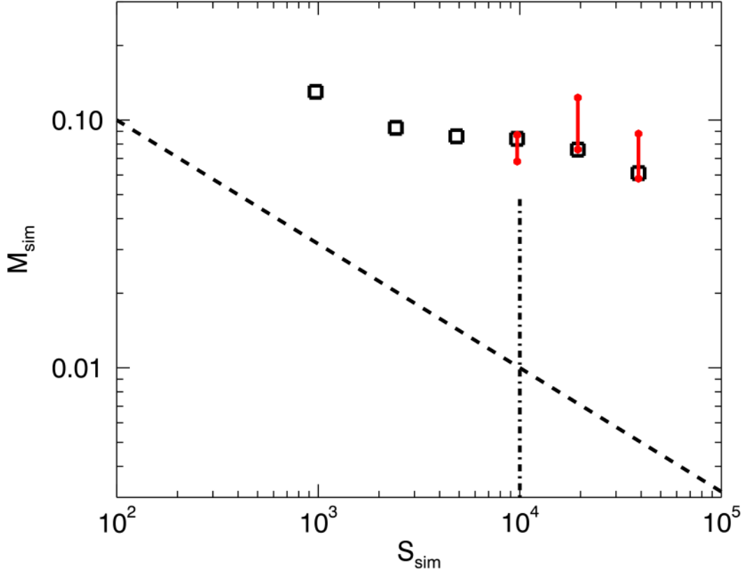
Fig. 6.— Normalized magnetic reconnection rate M_{sim} for 6 simulations with different Lundquist number ( S_{sim} ). The squares show the reconnection rate taken at a time in each simulation when the length of the current sheet has reached L_{sim} = 2.75L_0 , and in all simulations is before the onset of the plasmoid instability. The red lines show the range in reconnection rate taken again at later times in the three plasmoid-unstable simulations, after the plasmoids are formed. The dashed line is the Sweet-Parker scaling law M \propto 1/\sqrt{S} . The dot-dashed line shows the separation between plasmoid-stable and plasmoid-unstable regimes for these multi-fluid simulations, and is given by the value of S_{sim} where the power law fit of the simulation data \sigma_{sim}(S_{sim}) meets the \sigma_{sim} = 1/200 line in Figure 7.
