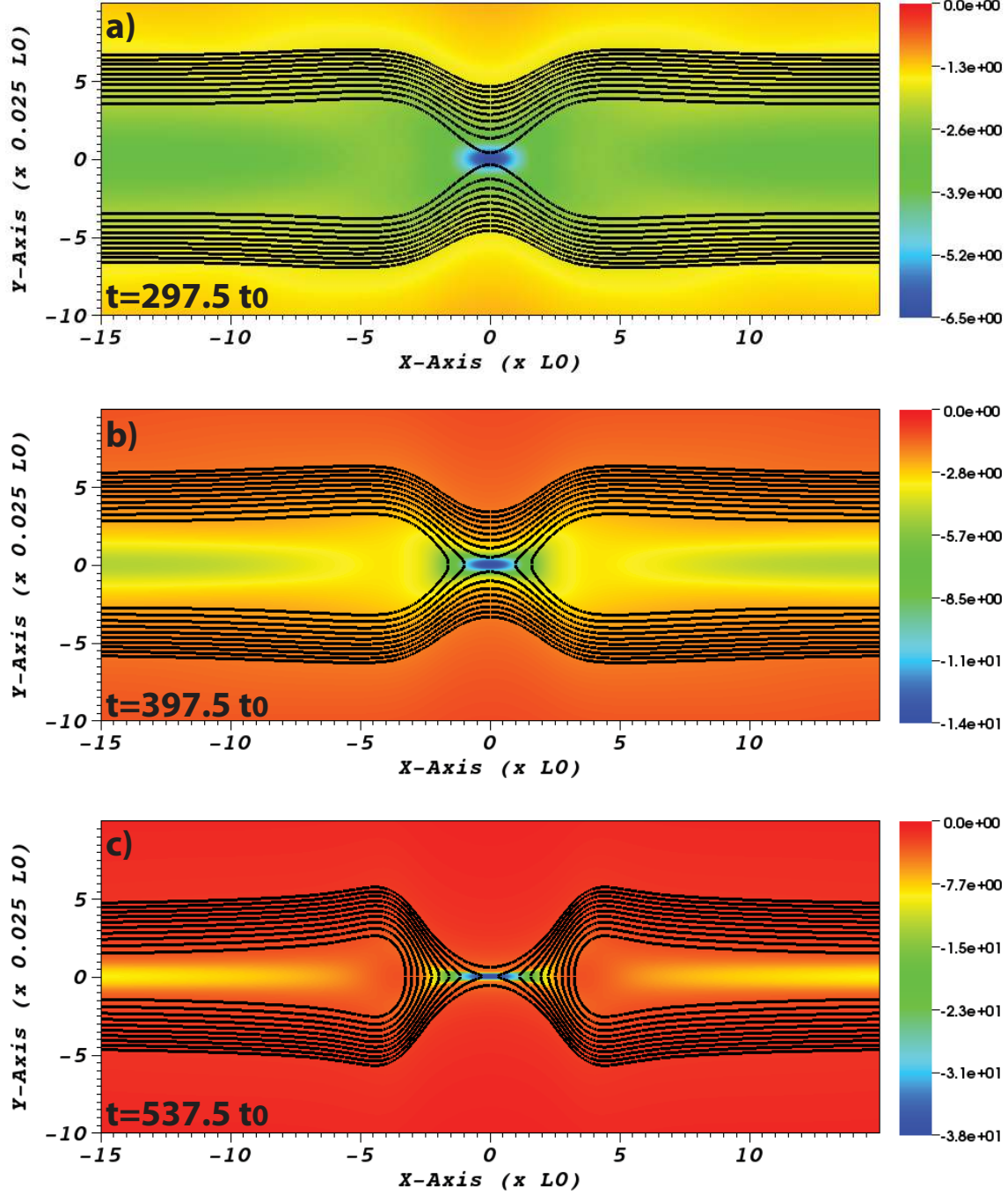
Fig. 2.— Formation of Sweet-Parker current sheet for the simulation where \eta = 0.5 \times 10^{-5} \eta_0 . Current density ( j/B_0/(\mu_0 L_0) ) is shown in the color contours, and 10 contour lines show A_z , evenly distributed in the interval [-0.04, -0.015]B_0 L_0 .
