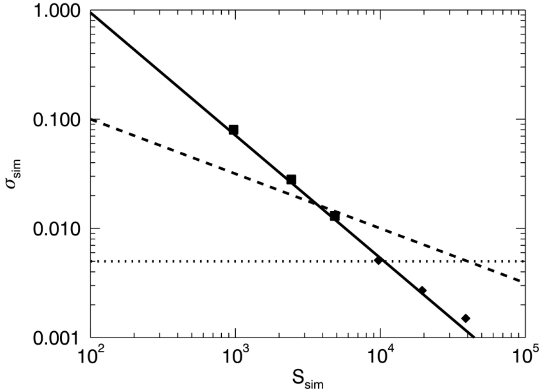
Fig. 7.— Scaling of simulation current sheet aspect ratio \sigma_{sim} with Lundquist number ( S_{sim} ). The squares are simulations where no secondary (plasmoid) instability is seen, and the diamonds are simulations where plasmoids are observed. The dotted line is the theoretical aspect ratio at which the plasmoid instability sets in. The dashed line is the Sweet-Parker scaling law ( \propto \sqrt{1/S} ). The solid line shows a line of best fit of the data to a power law. The exponent in the power law is -1.1 \pm 0.17 . This solid line intersects the \sigma_{sim} = 1/200 line at approximately S_{sim} = 10^4 .
