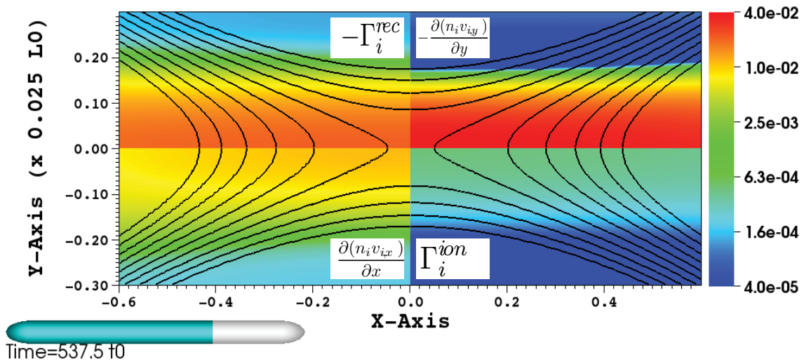
Fig. 4.— The steady state reconnection region showing contributing sources and sinks of ions in the current sheet (in units of L_0^{-3}t_0^{-1} ): Top left quadrant shows rate of loss of ions due to recombination. Bottom left quadrant shows rate of loss of ions due to outflow \frac{\partial n_i v_{ix}}{\partial x} . Top right shows rate of gain of ions due to inflow -\frac{\partial n_i v_{iy}}{\partial y} . Bottom right quadrant shows rate of gain of ions due to ionization. The solid lines are 10 contour lines of A_z , evenly distributed in the interval [-0.0378, -0.037]B_0L_0 . This shows that loss of ions due to recombination and outflow are comparable, and combine to balance the inflow of ions, with ionization playing an insignificant role.
