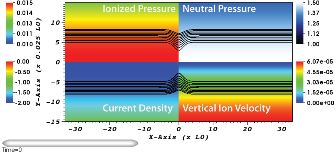
Fig. 1.— Initial conditions for a subset of the whole domain. Note that the y -coordinate is expanded by a factor of 40. The top left quadrant shows ionized pressure ( (P_i + P_e)/P_0 ), the top right quadrant shows neutral pressure ( P_n/P_0 ), the bottom left quadrant shows current density ( j/(B_0/\mu_0 L_0) ), and the bottom right quadrant shows vertical ion velocity ( v_{i,y}/v_0 ). The solid lines are 10 contour levels of the flux A_z evenly distributed in the interval [-0.04, -0.015]B_0L_0 .
