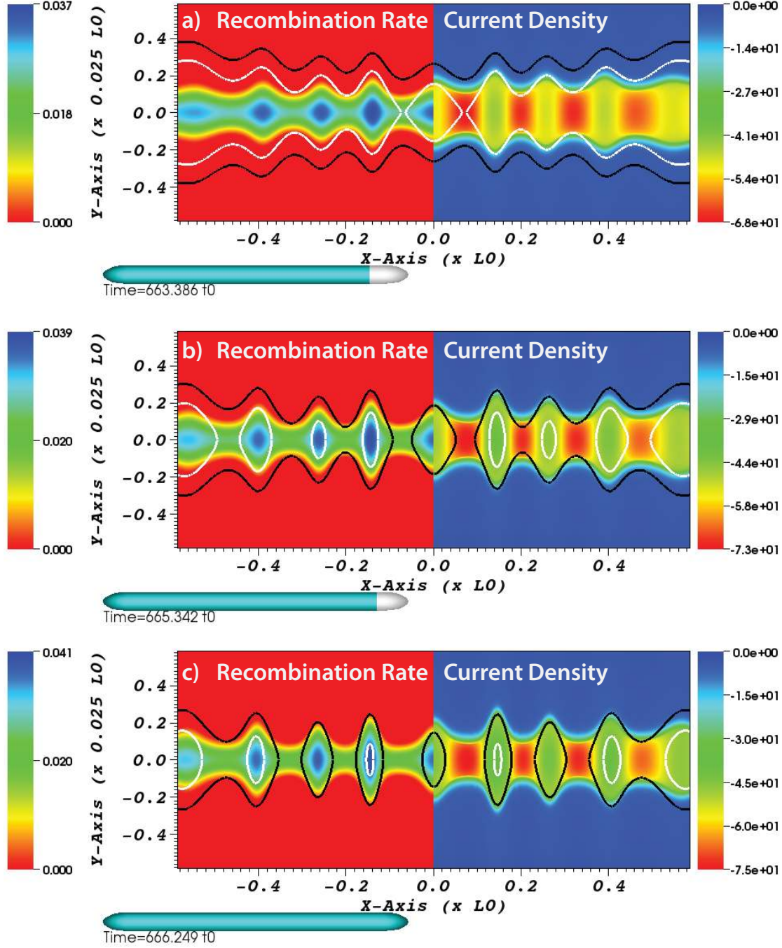
Fig. 8.— Plasmoid formation and evolution: Recombination rate \Gamma_i^{rec} L_0^3 t_0 (left) and current density j\mu_0 L_0/B_0 (right), and two contour levels of A_z of -0.0681B_0 L_0 (white) and -0.0687B_0 L_0 (black), at three different times in the simulation where \eta = 0.5 \times 10^{-5} \eta_0 .
