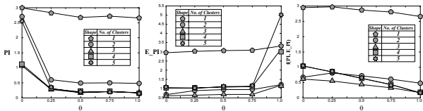
Fig. 8. Performance index of Multi-FNN treated as a function of the weighting factor for selected number of the clusters.
