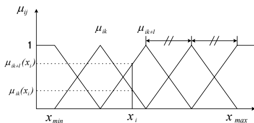
Fig. 2. MF definition before tuning (genetic optimization).
