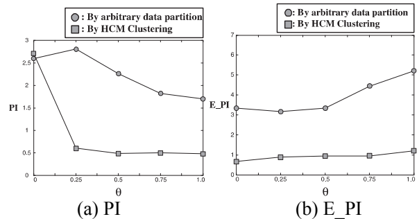
Fig. 7. Performance index of Multi-FNN treated as a function of \theta .
