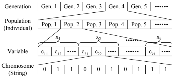
Fig. 6. Data structure of genetic algorithms for optimization of the FNN model.
