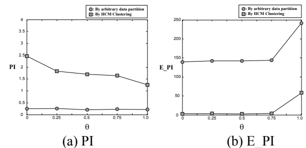
Fig. 9. Performance index of Multi-FNNs treated as a function of \theta .
