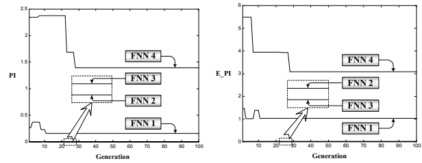
Fig. 11. Genetic optimization of the FNN model ( \theta=0.75 ).
