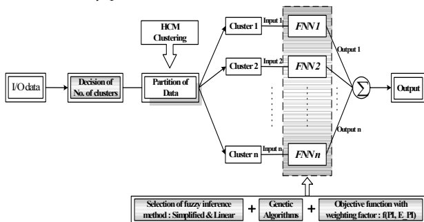
Fig. 3. Multi-FNN structure and ensuing development environment.
