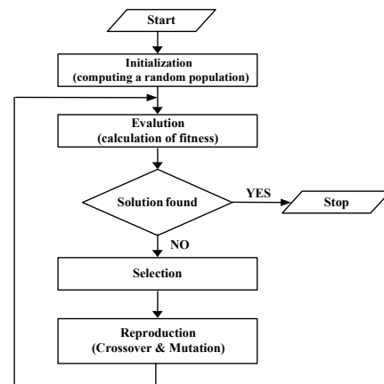
Fig. 5. A general GA flowchart.
