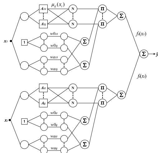
Fig. 1. Linear fuzzy inference-based basic FNN structure.
