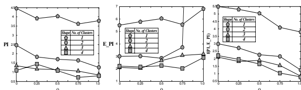
Fig. 10. Performance index of Multi-FNNs treated as a function of the weighting factor for a selected number of the clusters.
