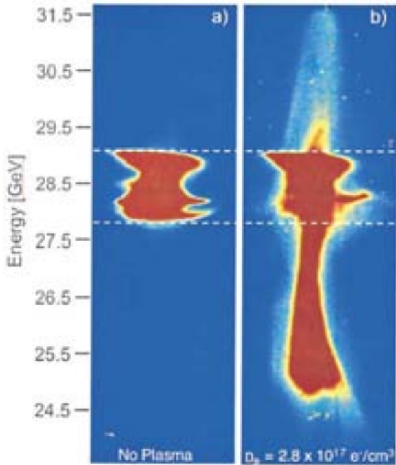
FIG. 2 (color). Single bunch energy spectra downstream from the plasma for (a) the case of no plasma and (b) a 10 cm long 2.8 \times 10^{17} e^-/\text{cm}^3 lithium plasma. The no plasma case shows the \sim 1 GeV energy spread typical of the incoming compressed pulses. At right, the core of the electron bunch has lost energy driving the plasma wake while particles in the back of the bunch have been accelerated to 2.7 GeV over the maximum incoming energy. The images are displayed with a saturated color map to highlight the 7% of the bunch particles accelerated to energies higher than the maximum incoming energy. The peak intensity in both figures is more than a factor of 4 below the saturation level of the camera.
