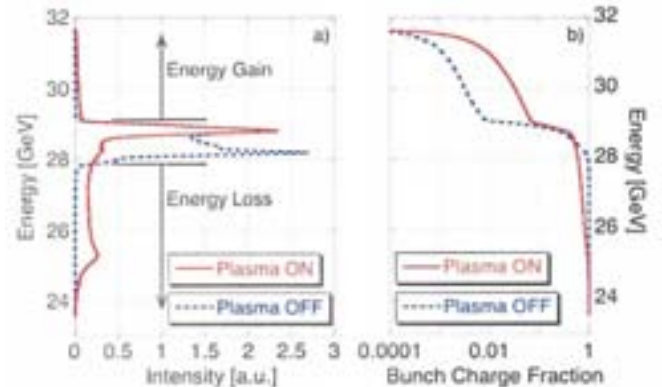
FIG. 3 (color). (a) Energy spectra for a plasma on and off case. 25% of the electrons in the head of the bunch, which also have the highest energies in the plasma off case, are not affected by the lithium vapor. (b) The normalized cumulative charge sum is used to quantify the energy gain or loss of the highest or lowest energy 1% fraction of bunch particles.
