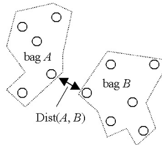
Figure 1: An intuitive way to define the distance between bags
