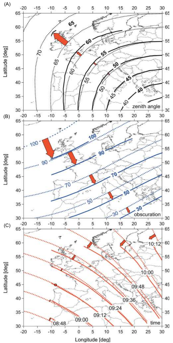
Fig. 16. Differences in eclipse geometry (Earth's curvature ignored) at ground level (dashed curves) and ionospheric height of 300 km (solid curves): zenith angle (A), obscuration (B), and time (C) at the eclipse maximum. The changes in geometry, going from sea level to ionospheric height, are highlighted by using (red) arrows.
