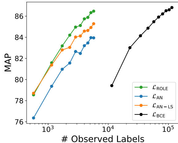
Figure 1. It is possible to approach the performance of full supervision ( \mathcal{L}_{BCE} ) using only one positive label per image. Here we show test MAP as a function of the number of training labels for PASCAL VOC 2012 [13]. Each curve is generated by randomly subsampling m\% of the images from the training set for m \in \{10, 20, \dots, 100\} . The number of labels per image then determines the number of observed label on the horizontal axis: \mathcal{L}_{BCE} receives all 20 labels per image, while the other methods only receive one positive label per training image. Despite having a factor of 20 times fewer labels, our \mathcal{L}_{ROLE} approach achieves comparable performance to the fully labeled case ( \mathcal{L}_{BCE} ).
