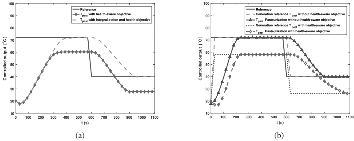
Fig. 8. Evolution of pasteurization temperature T_{past} with and without the health-aware objective in MPC: pasteurization temperature T_{past} in a single-layer (a), pasteurization temperature T_{past} in a multi-layer (b).
