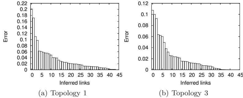
Fig. 2. Error rates of inferred overlay links
