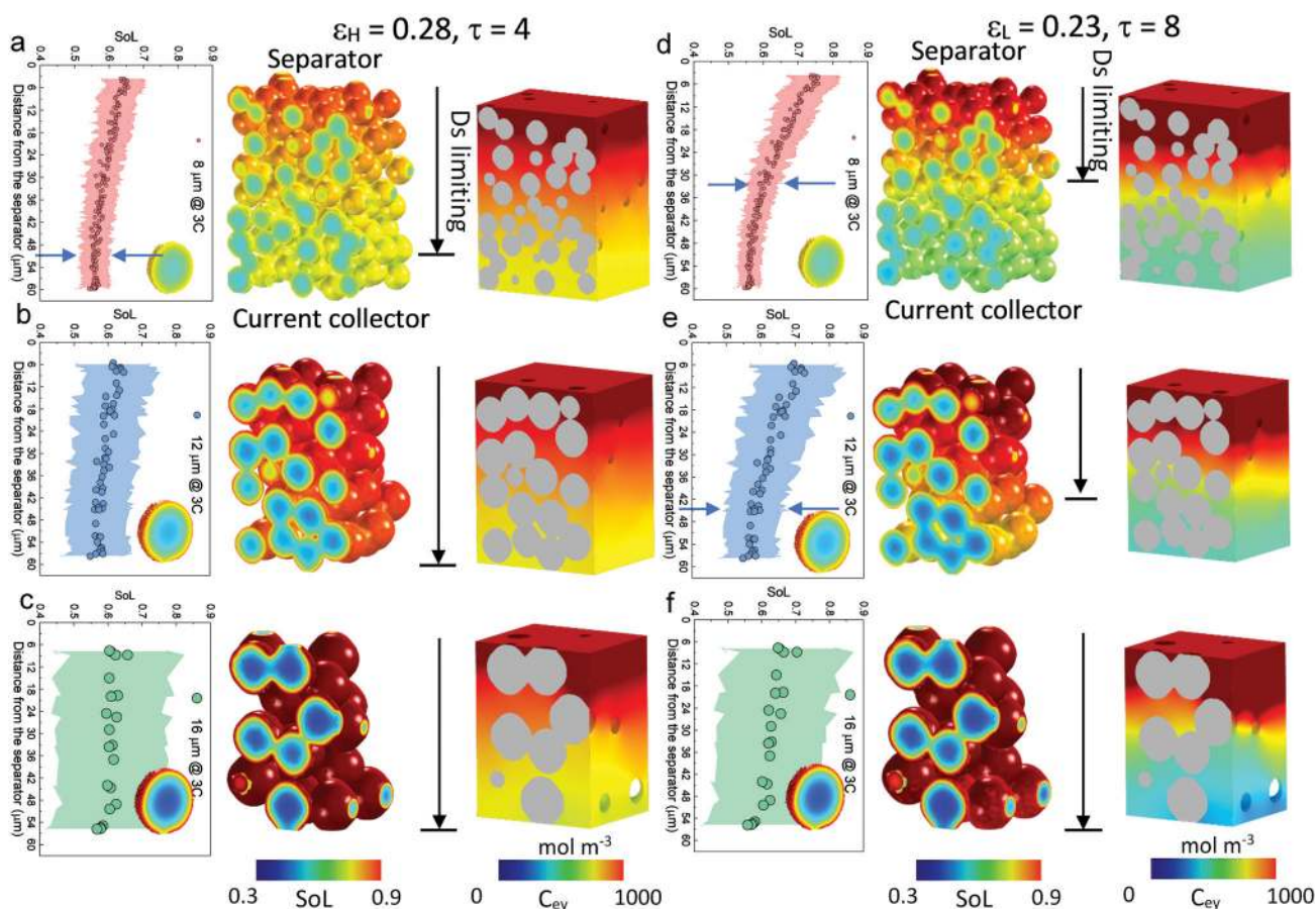
Fig. 3 Electrochemical simulation (3C discharge, half cell NMC vs. Li anode) in (a) D8 (b) D12 and (c) D16 at high porosity ( \epsilon_{\text{H}} ) and (d) D8 (e) D12 and (f) D16 at low porosity ( \epsilon_{\text{L}} ), respectively. The average SoL and its standard deviation within each particle are plotted alongside each electrode at 60% DoD. The inset in each plot presents the single-particle simulation, regarded as a reference to determine the Ds limiting region. Ds varies with SoL, as shown in Fig. S8 (ESI † ).
