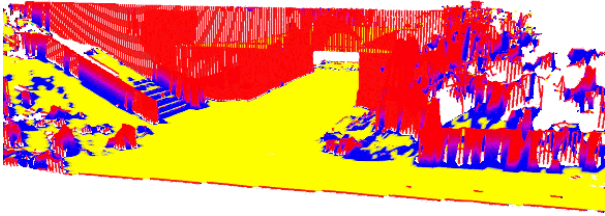
Fig. 3. Classification result for the MLS map depicted in Figure 1(d). The three colors/grey levels indicate the classification result for the individual surface patches into traversable, non-traversable, and vertical ones.
