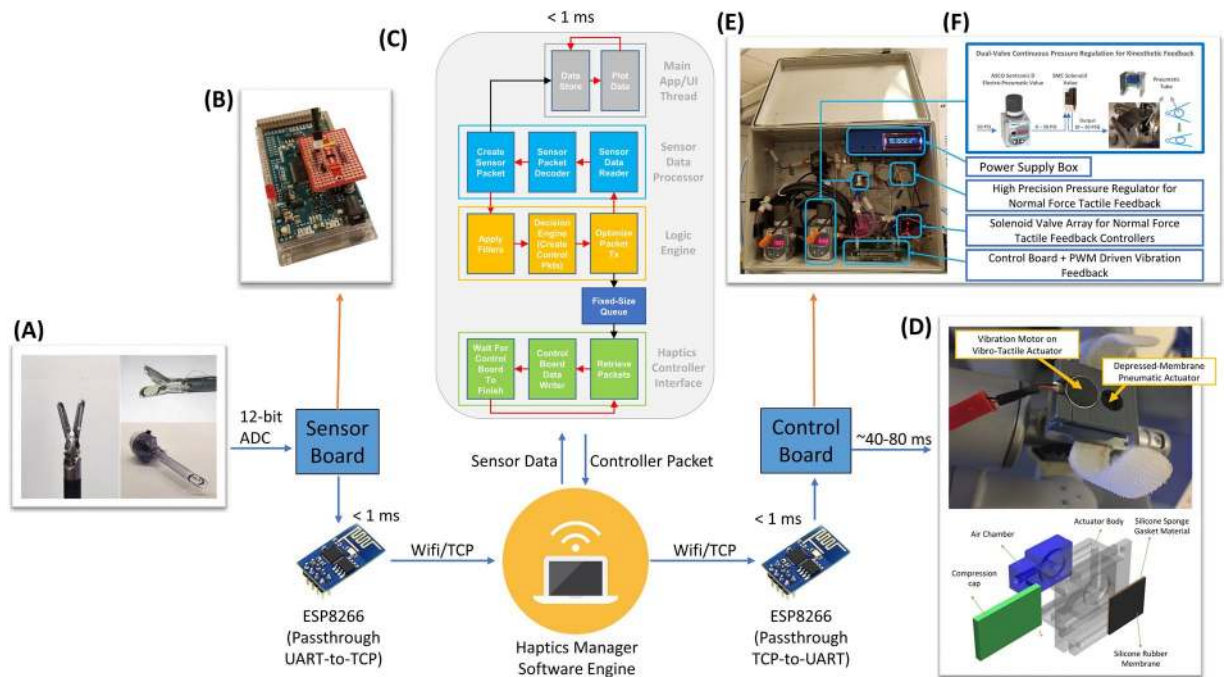
Figure 4. Multi-Modal HFS system architecture, Average component delays marked in milliseconds. (A) Sensors mounted on da Vinci instruments. Da Vinci Cadiere grasper measuring 5 mm × 14 mm shown on the left. Cadiere graspers with pressure sensors installed on the top right and 12 mm Trocar 47–49 on the bottom right. (B) Sensor board. (C) Haptics Manager Software Architecture. (D) CAD model of 3D-printed depressed membrane tactile actuator and the tactile feedback actuator mounted on da Vinci controls. (E) Multi-Modal HFS Control hardware. (F) Dual-Valve pressure regulation system for use with the modified 3D-printed actuators (w/pneumatic tube for providing kinesthetic force feedback).
