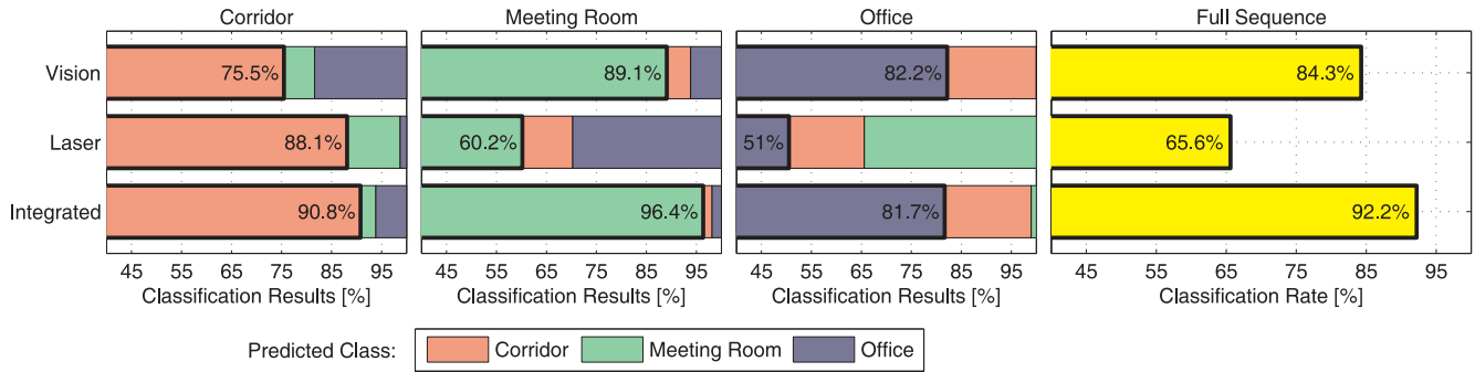
Fig. 18. Place classification results obtained on the dataset recorded during the test run. The first three bar charts show the results separately for each place class: “corridor”, “meeting room” and “office”. The charts show the percentage of the samples that were properly classified (most left bars marked with thick lines), but also how the misclassifications were distributed. The chart on the right presents the percentage of properly classified samples during the whole run. The two top rows give results for single modalities, while the bottom row shows results for the multi-modal system.
