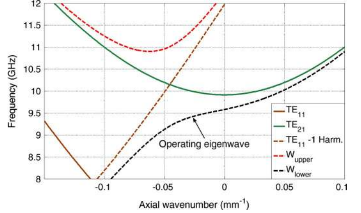
Fig. 1. Coupling between the TE_{21} mode and the spatial harmonic TE_{11} mode in a three-fold helical waveguide.
