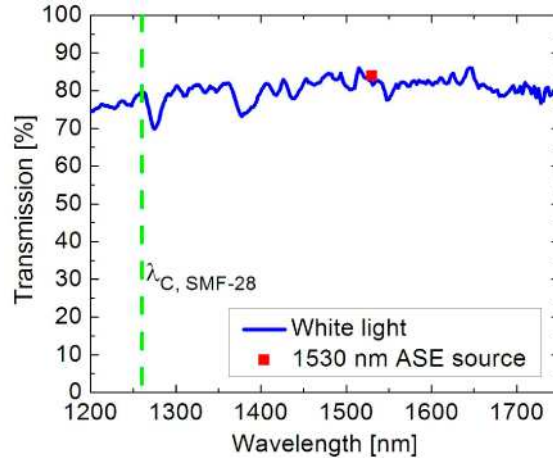
Fig. 6. Spectral transmission loss through two Photonic Lanterns spliced back-to-back (solid blue line). Light is coupled into device #1 with the 95 \mu\text{m} core MM fiber with 95% of the power in an NA below 0.09. The 0.76 dB transmission loss measured with a 1530 nm ASE source is shown by the red square. The dashed green line indicates the higher-order mode cut-off wavelength of the SMF-28 fibers.
