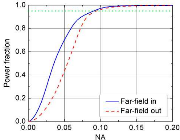
Fig. 5. Measured integrated far-field coupled into device #1 (solid blue line) and resulting far-field out of device #2 (dashed red line).
