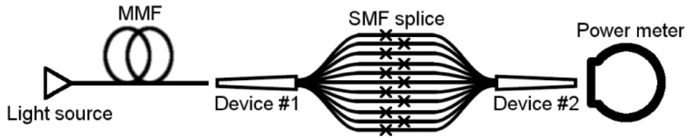
Fig. 4. Schematic illustration of the setup used to characterize two Photonic Lanterns coupled back-to-back.
