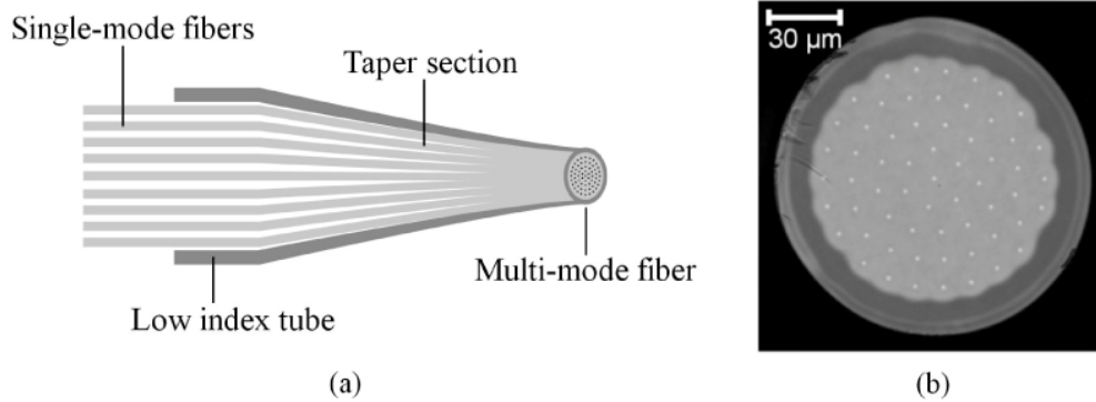
Fig. 2. (a) Schematic illustration of the fabricated Photonic Lantern. (b) Microscope image of the cross section of the MM tip of the Photonic Lantern.
