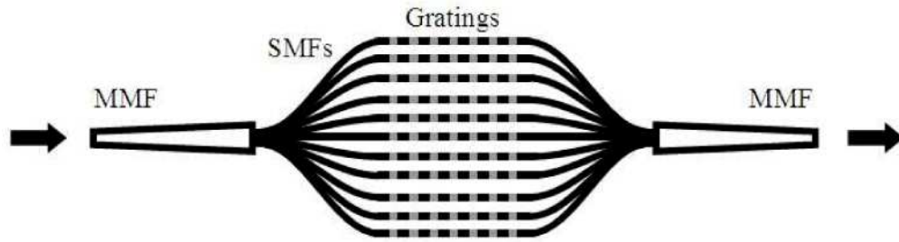
Fig. 1. Schematic illustration of an optical system with two Photonic Lanterns in a back-to-back configuration and fiber Bragg gratings in each of the SMF ports.
