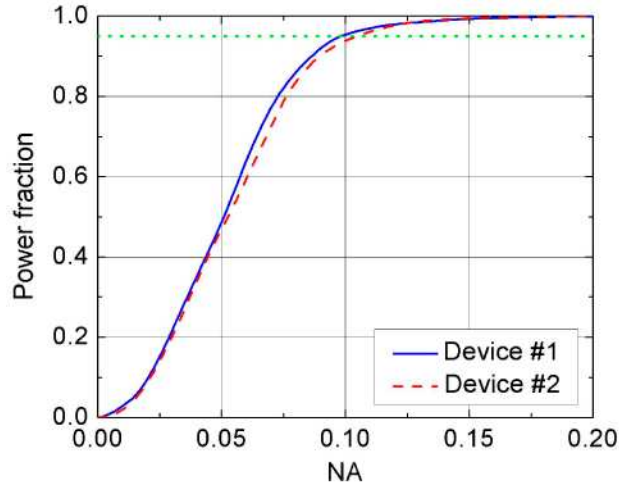
Fig. 3. Measured integrated far-field out of the MM end of the Photonic Lanterns. The far-fields are averaged over 10 measurements made with light coupled into 10 randomly chosen SM ports one at the time.
