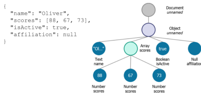
Fig. 10. An example of modeling JSON data as trees in MarkLogic (source: https://developer.marklogic.com/features/json )
