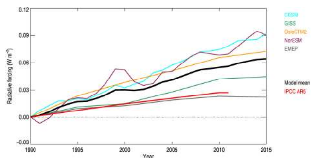
Figure 7. Radiative forcing ( \text{W m}^{-2} ) due to the change in ozone over the period 1990–2015.
