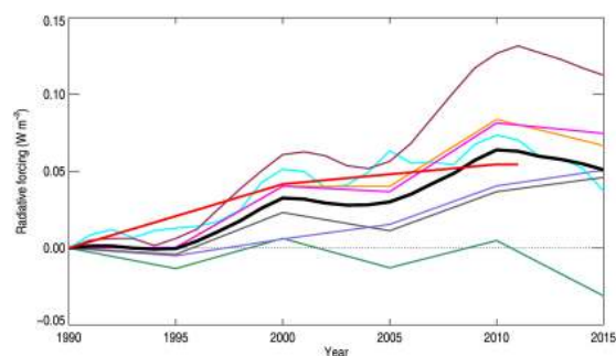
Figure 3. Radiative forcing ( \text{W m}^{-2} ) of the direct aerosol effect over the period 1990–2015 given for seven models (legend lists the models); the multi-model mean is shown in black and the estimate provided in IPCC AR5 is included in red.
