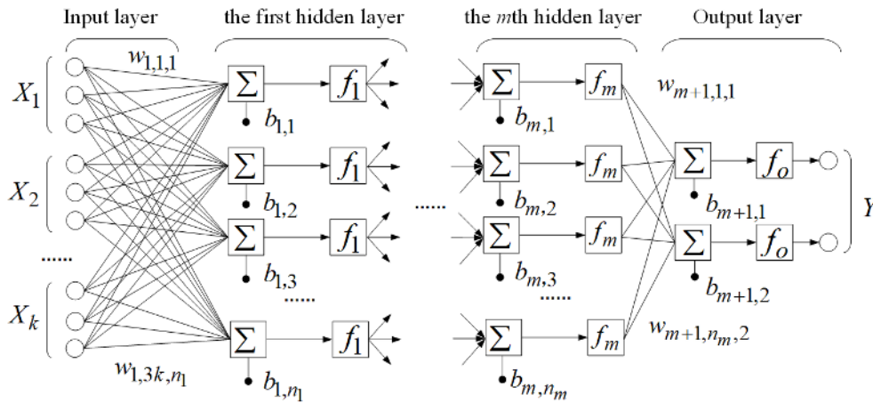
FIGURE 5. Structure of neural network for conducted emission suppression evaluation.
