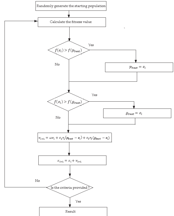
Figure 1 PSO flow diagram
