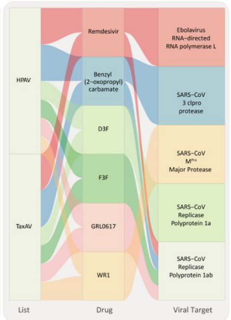
b Selected drugs targeting viral proteins
