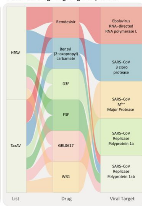
b Selected drugs targeting viral proteins
