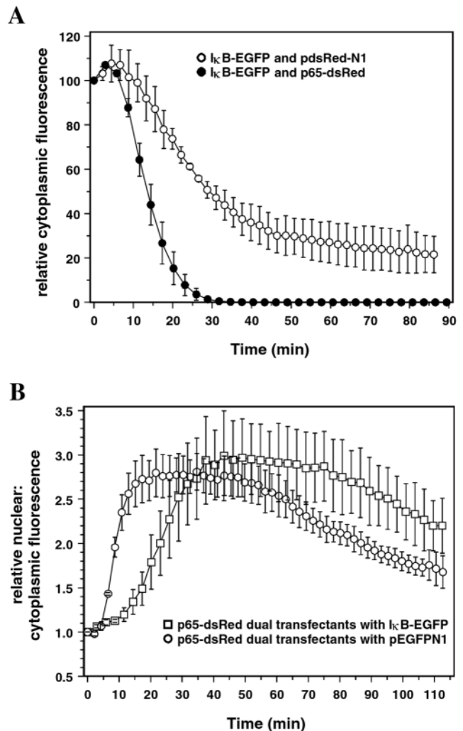
Fig. 3. Combined imaging of p65-dsRed localisation and I \kappa B \alpha -EGFP degradation following TNF \alpha stimulation of dual-transfected cells. (A) Quantification of I \kappa B \alpha -EGFP degradation in dual-transfected cells also expressing either p65-dsRed or the control expression vector pdsRedN1. I \kappa B \alpha -EGFP fluorescence was determined as described in Fig. 2. (B) Quantification of translocation of p65-dsRed in dual-transfected cells also expressing either I \kappa B \alpha -EGFP or the control EGFP-N1. The nuclear:cytoplasmic ratio of p65-dsRed fluorescence was determined as described in Fig. 1. Results show mean values \pm s.d. ( n-1 ) from two experiments, using at least four cells from each experiment.
