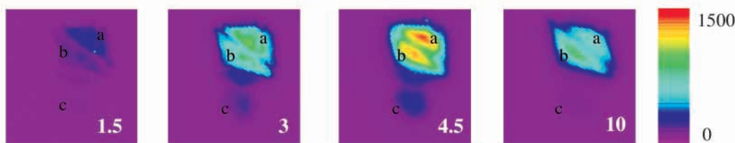
C Cellular luminescence after confocal microscopy following TNF \alpha (time shown in h after TNF \alpha )
