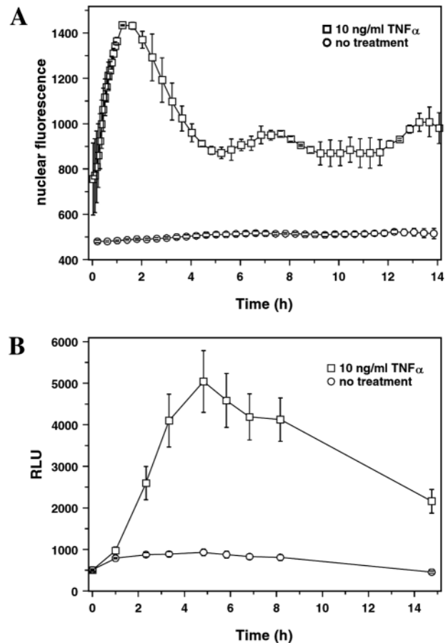
Fig. 5. Long term NF- \kappa B response to TNF \alpha . (A) Long term widefield fluorescence microscopy of p65-localisation in response to TNF \alpha . Cells were treated at t=0 hours with 10 ng/ml TNF \alpha or carrier (control). Mean nuclear fluorescence intensities were determined for each cell at each time point. Results show mean values obtained from two experiments. (B) Transcriptional regulation of NF- \kappa B-sensitive promoter. Luciferase expression monitored in living cells transfected with pNF- \kappa B-luc. Cells were transfected in 24-well microtitre plates. 1 mM luciferin was added to cells 12 hours prior to addition of TNF \alpha (10 ng/ml final concentration) or carrier added at t=0 hours [ n=4 , results show means \pm s.d.( n-1 )].
