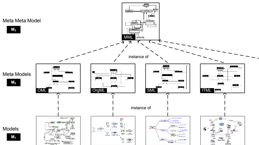
Fig. 2 MEMO Language Architecture
