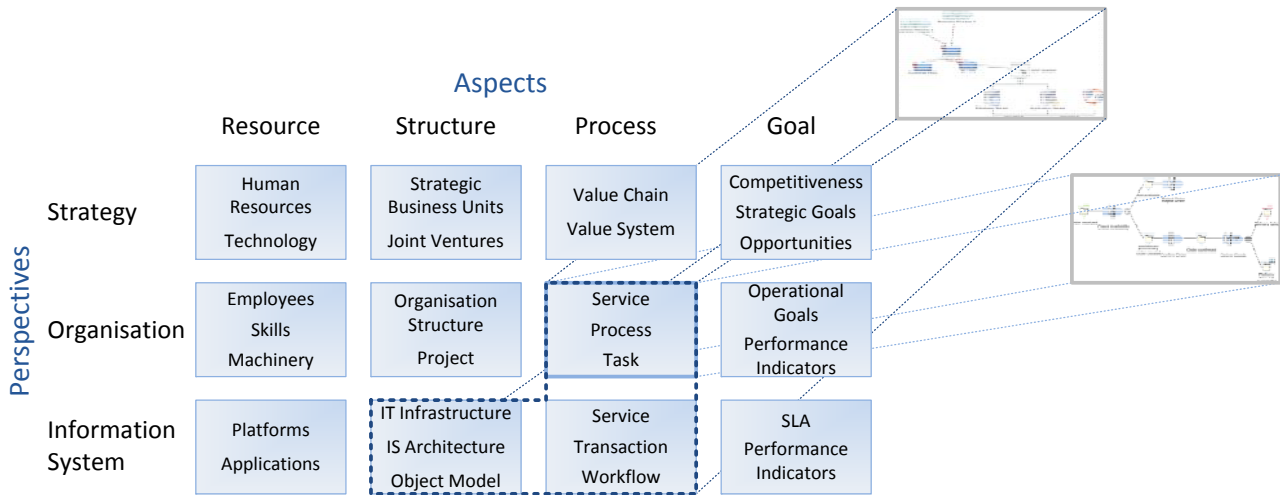
Fig. 1 High-Level Framework for Structuring the Enterprise and associated Diagram Types
