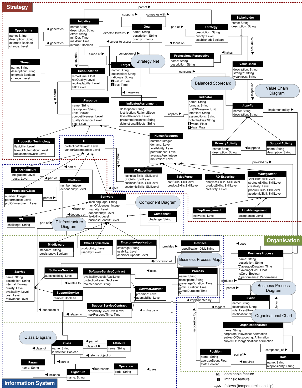
Fig. 4 Excerpt of Integrated Meta Models
