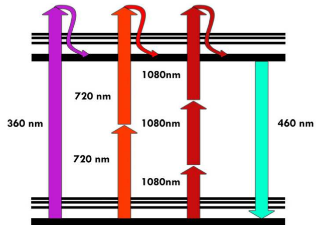
Figure 1 Perrin-Jablonski fluorescence diagram. Simplified Perrin-Jablonski scheme for 1PE, 2PE and 3PE. Once the excited state has been reached the subsequent fluorescence emission is the very same for the three different modalities of excitation.
