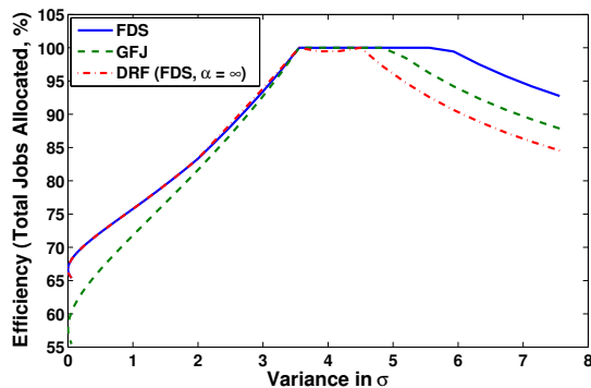
Fig. 10. Greater variance in \sigma leads to DRF inefficiency in the number of jobs processed: Percentage efficiency versus variance in user heterogeneity in a datacenter example.
