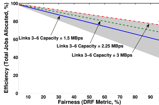
Fig. 20. Attainable efficiency vs. fairness for \beta \in (-5, 5) and \lambda \in (0.01, 1.91) for \beta < 0 , \lambda \in \left(0.005 \left(\frac{1}{\beta} - 2\right), 0.955 \left(\frac{1}{\beta} - 2\right)\right) for \beta > 0 values in a bandwidth allocation example, using FDS. DRF is used as the fairness benchmark and metric.
