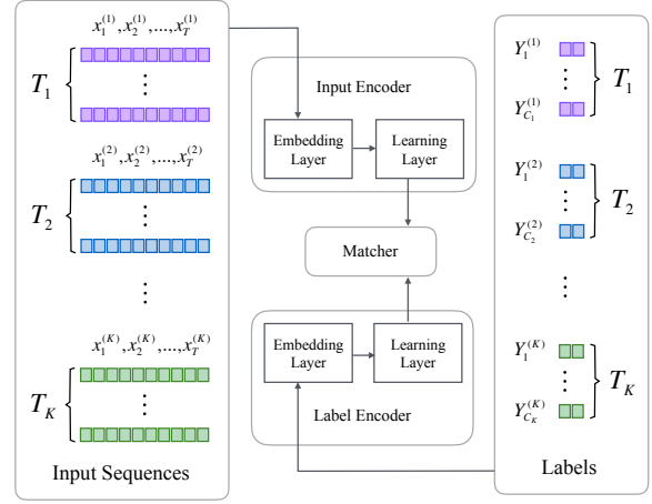
Figure 1: General Architecture of MTLE
