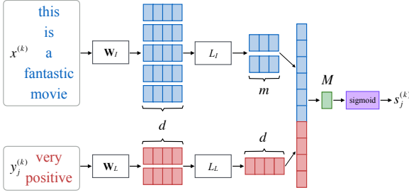
Figure 2: Implementation Details of MTLE
