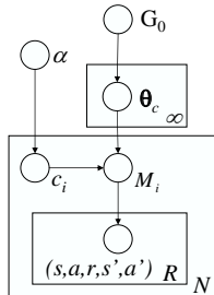
Figure 2. Infinite Mixture Model (Parameter set \Psi ). There are N MDPs. For each MDP the agent has made R observations. Parameters \theta_c capture the class distributions (level 2 in Figure 1) and the parameter set G_0 is a hyperprior over classes (the root in Figure 1). The class assignments c_i assign each MDP to a class. The parameter \alpha influences the probability with which new classes are considered.
