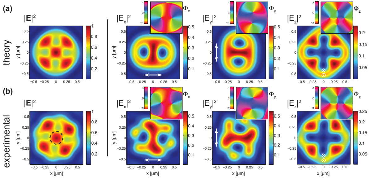
Figure 3. Electric energy density distributions of a tightly focused structured beam. (a) Numerically calculated focal field distribution for a tightly focused composite beam generated from a coherent superposition of \text{LG}_{0,0}(\rho, \phi, z) \hat{\mathbf{e}}_R and \text{LG}_{0,2}(\rho, \phi, z) \hat{\mathbf{e}}_L . The total electric energy density distribution is plotted on the left, while the individual Cartesian components as well as their relative phase distribution are depicted on the right. (b) Experimentally reconstructed focal field distribution of the same input field used in (a), showing the very good overlap between experiment and calculation. All distributions are normalized to the maximum value of the corresponding total electric energy density distribution.
