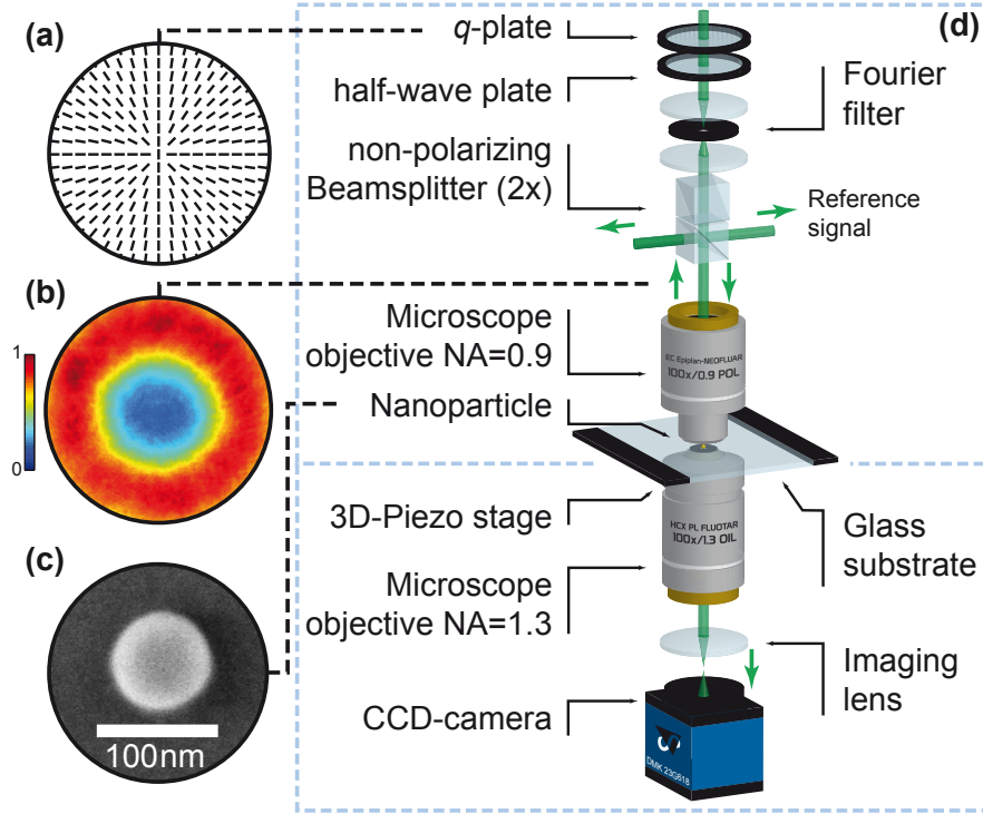
Figure 2. Sketch of the experimental setup. (a) Distribution of the local fast axis of the liquid crystal molecules in the transverse plane of the employed q = 1 -plate. (b) Experimentally generated intensity distribution of the resulting full-Poincaré beam that is subsequently focused. Note that a half-wave plate is used to transform the output polarisation topology into that of a q = -1 -plate. (c) SEM-image of the utilized gold nano-sphere with a diameter of 80 nm. (d) Sketch of the experimental setup utilized to reconstruct the full vectorial focal field distribution of the tightly focused full Poincaré beam.
