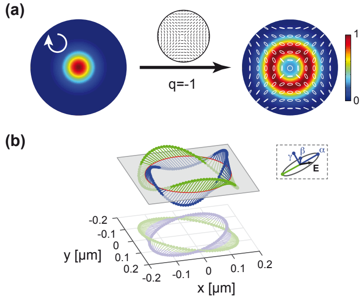
Figure 1. Creation of a full Poincaré beam and subsequent optical polarization ribbon with twist index -2 under tight focusing. (a) A left-handed circularly polarized Gaussian beam is converted into a full Poincaré beam by means of a space-variant birefringent plate ( q -plate) with topological charge q = -1 (see sketch for the orientation of its fast axes) and optical retardation of \delta = 2.92 rad. The resulting polarization ellipse at each point in the transverse plane of the beam is superimposed in white. (b) Twisted ribbon with 2 twists and its projection onto the transverse plane, created by tight focusing of the beam shown in (a) and tracing the major axis \alpha of the polarization ellipse (see inset for a sketch with the definition of its parameters) on a circle with \rho = 150 nm around the optical axis.
