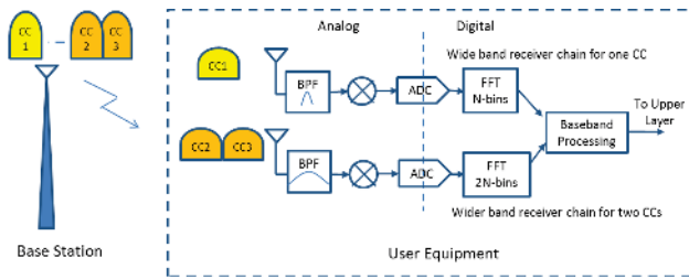
Figure 3. User equipment with multiple receiver chains
