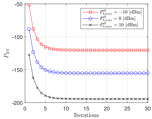
FIGURE 5. P_{RS} function convergence plot with increasing number of algorithm iterations, where K = 4 and P_{0,max}^{dl} = -10\text{dB}, 0\text{dB}, and 10\text{dB} .
