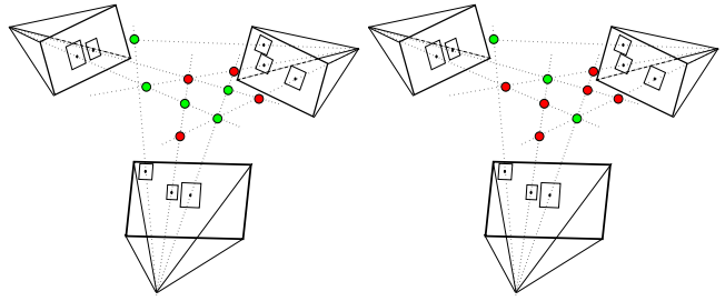
Fig. 10 MDL principle - the corresponding pairs generate 3D hypotheses, from which can be picked up (green) a subset (left) or the best/smallest subset (right) in the MDL sense that explains the 2D detections.
