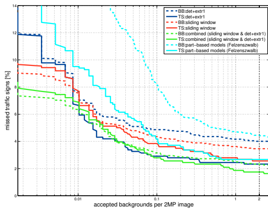
Fig. 11 Comparison with state-of-the-art methods. - Detection plots for every time a sign appears ( BB - bounding box level), or only demanding it is detected at least once ( TS - traffic sign level). In blue one finds results for the main pipeline presented in this paper. The results for the alternative sliding window approach are shown in red. Green shows results for their combined use. The combined performance is better than the sliding window approach and our proposed approach with Extr1 extraction setting taken alone. In cyan is the result of the generic part-based model system from Felzenszwalb et al. [8]
