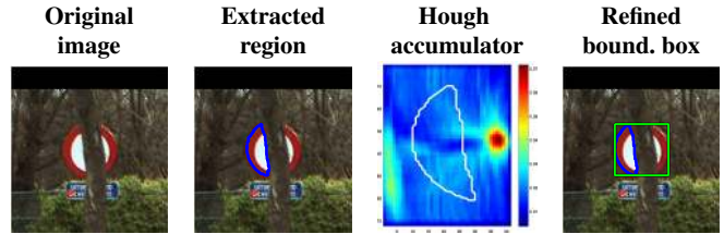
Fig. 7 Shape-based extraction principle. The border of the colour-based extracted region (blue) votes for different shapes in a Hough accumulator. The green bounding box corresponds to the maximum.
