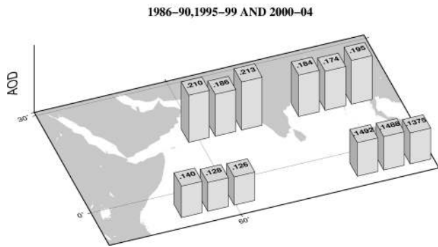
Fig. 2. The mean AVHRR AOD for all four regions for the period 1986–1990, 1995–1999 and 2000–2004. The mean value is written on the top side of the column.
