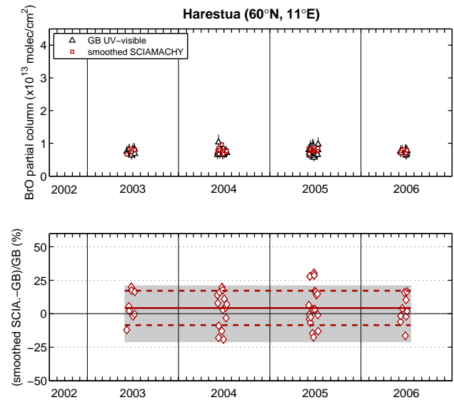
Fig. 12. Comparison of the 18–27 km BrO partial columns calculated from the smoothed SCIAMACHY limb and ground-based UV-visible profiles at Harestua (60° N, 11° E) for the 2002–2006 period (evening coincidences). The relative differences appear on the lower plot. The error bars on the ground-based data correspond to the total error (systematic error + total retrieval error), estimated as in Hendrick et al. (2007). The solid and dashed red lines in the lower plot correspond to the mean relative difference and its one-sigma standard deviation, respectively. The grey-shaded area indicates the mean uncertainty region for the ground-based UV-visible partial columns.
