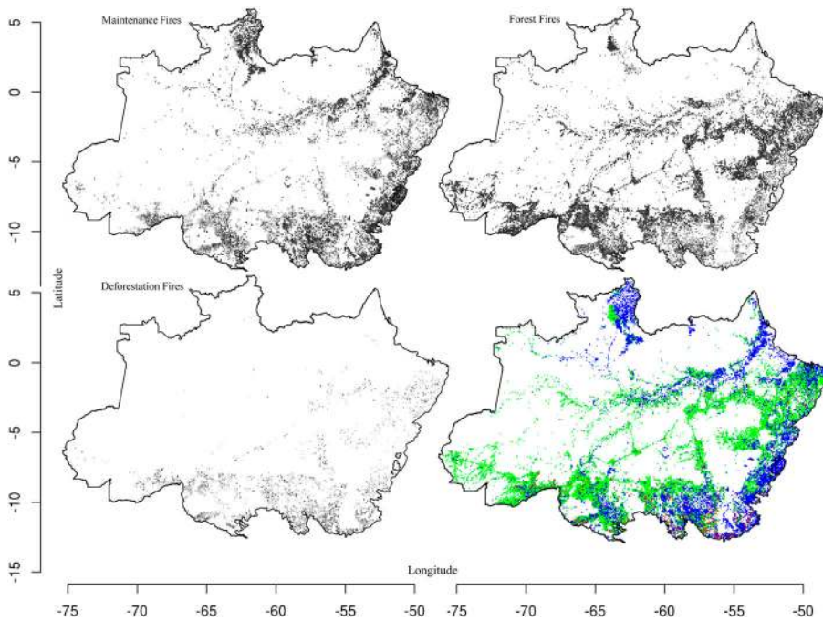
Figure 8. 2003 fire type classification results showing the majority classified fire type in 7 km \times 7 km grid cells colored as maintenance fires (blue), forest fires (green), and deforestation fires (red). The grayscale images show the relative proportion of the active fire detections classified into each fire type in each grid cell (white = 0; 0 > light gray \leq \frac{1}{3} ; \frac{1}{3} > medium gray \leq \frac{2}{3} ; \frac{2}{3} > dark gray \leq 1). A total of 201,519 (Figure 2) classified MODIS active fire detections are shown.
