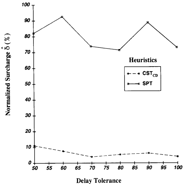
Fig. 11. Normalized surcharge \delta versus delay tolerance for the number of nodes=50 and group size=20, with average degree of each node=10, w.r.t. CST_C .
