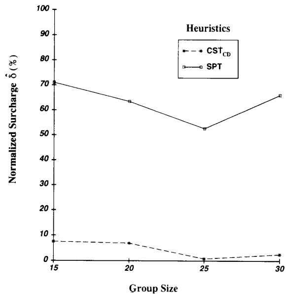
Fig. 10. Normalized surcharge \hat{\delta} versus group size, for number of nodes=60 and \Delta=80 , with average degree of each node=5, w.r.t. CST_C .
