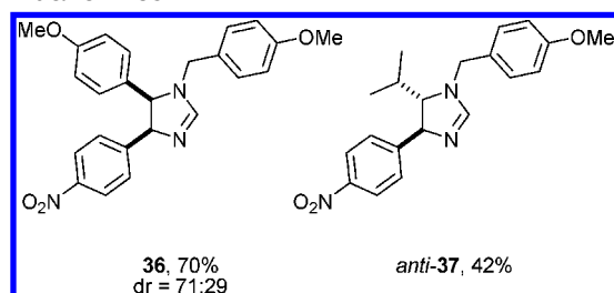
CHART 1. 4-Nitrophenyl-Substituted 2-Imidazolines
