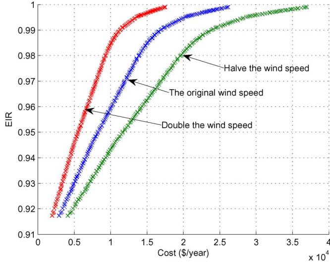
Fig. 7. Impacts of different wind speeds on derived Pareto fronts.
