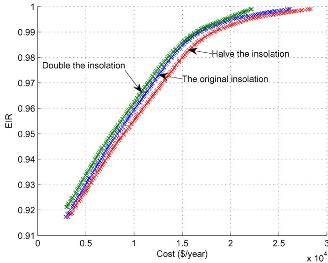
Fig. 8. Impacts of different insulations on derived Pareto fronts.
