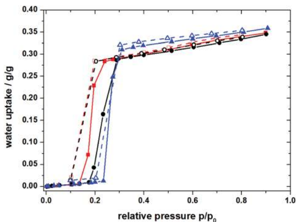
Fig. 2 Water ad-/desorption isotherm of CAU-10-H at different temperatures. 25 °C adsorption —■—, 25 °C desorption - -□-, 40 °C adsorption —●—, 40 °C desorption - -○-, 60 °C adsorption —▲—, 60 °C desorption - -△-.
