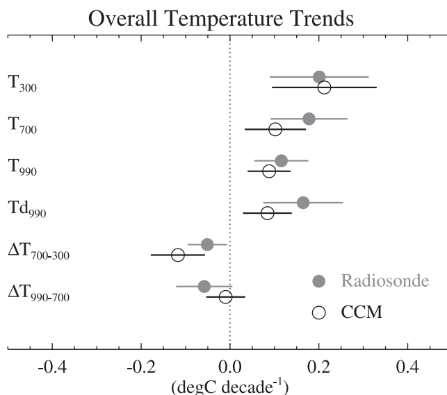
Figure 5. Overall tropical radiosonde (solid circles) and CCM (open circles) trends (in degC decade -1 ) for temperature at 300 hPa (T 300 ), temperature at 700 hPa (T 700 ), temperature at 990 hPa (T 990 ), dew-point temperature (Td 990 ), temperature difference 700–300 hPa (T 700-300 ), and temperature difference 990–700 hPa (T 990-700 ). Trends are indicated by the circle, and the 95% confidence interval is indicated by the horizontal bar.
