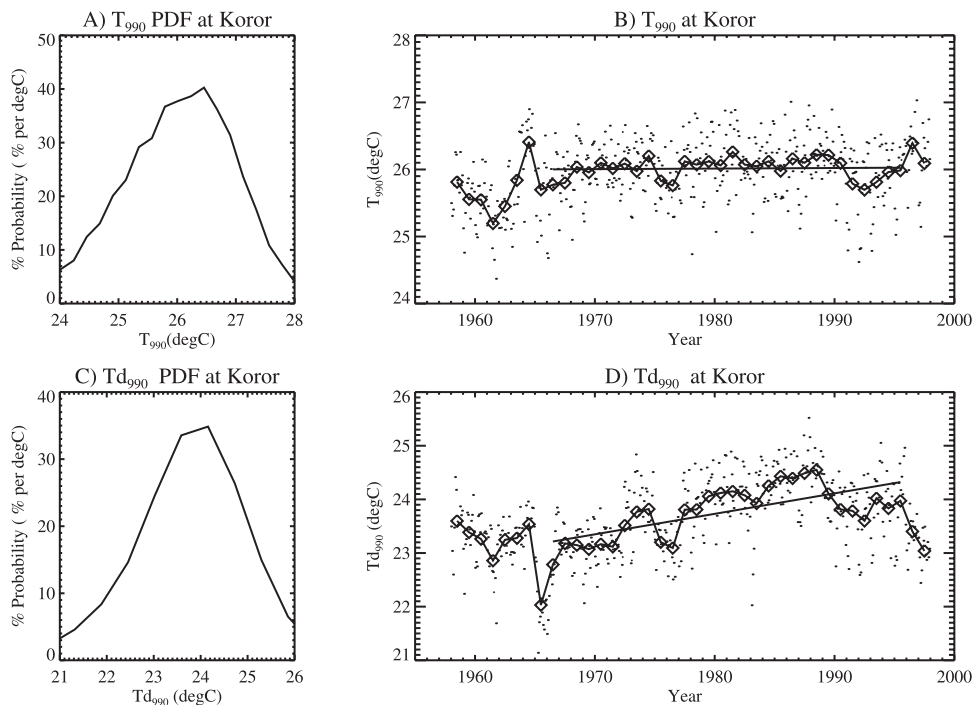
Figure 1. Thermodynamic trends for Koror. (a, b) Temperature at 990 hPa. (c, d) Dew-point temperature at 990 hPa. Left-hand panels are PDFs in percent and right-hand panels are monthly (points) and annual (diamonds) means. Straight line is a linear trend fit to the annual means.
