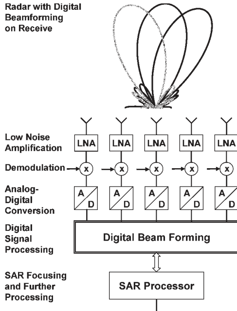
Fig. 1. Schematic of digital beamforming on receive. The signal from each subaperture element is independently amplified, down-converted, and digitized. The digital processing enables flexible and adaptive beamforming after signal reception.
