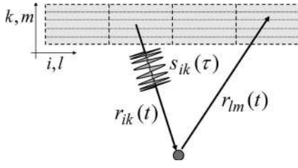
Fig. 11. Signal model for the response of a multiaperture Tx/Rx system to an isolated point scatterer.
