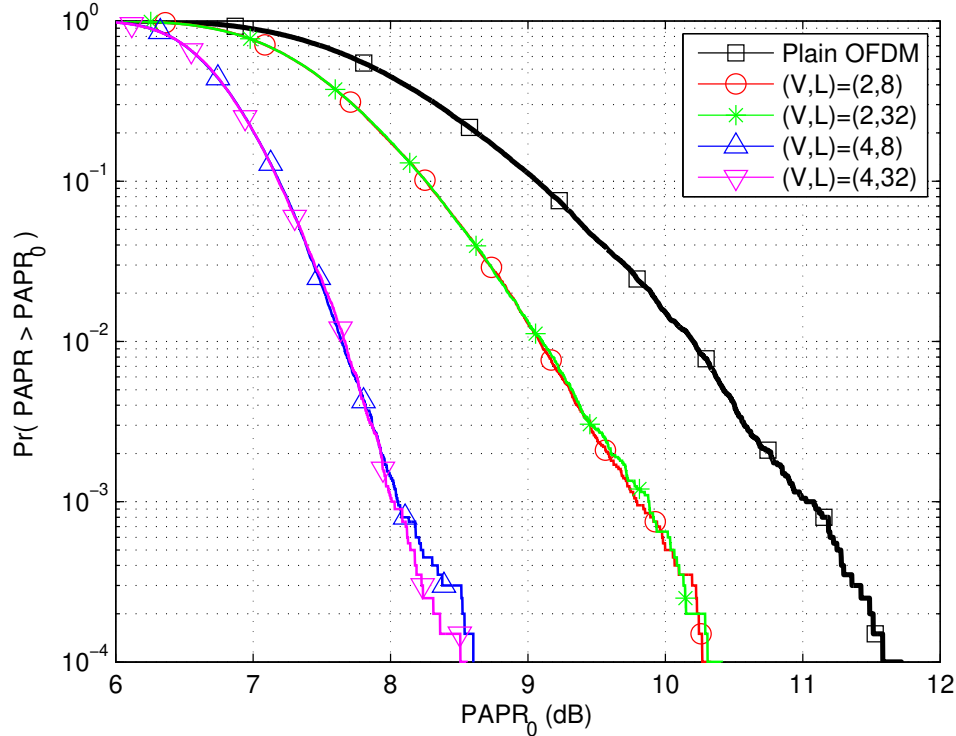
Figure 5.6 The effect of block sizes on PAPR.
