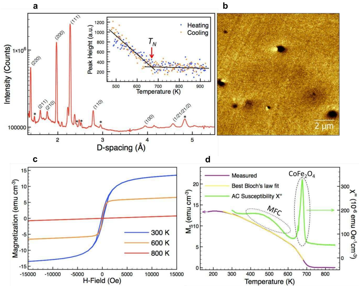
Figure 4. Magnetic characterisation of BFC-BKT ceramics. a , Neutron diffraction pattern of polycrystalline ceramic at room-temperature (logarithmic intensity scale). Peak height of magnetic ( 1/2 ) 1/2 ) peak vs. temperature (inset) indicates T_N = 670 \pm 10 K. This extremely high T_N might be attributed to MFC. Peaks due to \text{CoFe}_2\text{O}_4 phase are marked by *. b , MFM phase image showing typical MFC. c , Magnetization vs. magnetic field (M-H) loops T = 300, 600 and 800 K. d , The spontaneous magnetization, M_S \approx 2 M(25 kOe)-M(50 kOe) vs. T (—) is best-fitted by Equation (1) between 250 and 680 K (---). Imaginary part of AC susceptibility ( \chi'' ) vs. T (—, H_{AC} = 10 Oe, f = 23 Hz) reveals two peaks at 471.8 and 673.7 K which are correlated with the Curie temperatures of two different magnetic components, MFC and \text{CoFe}_2\text{O}_4 .
