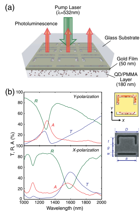
FIG. 1 (color online). (a) Schematic of a plasmonic metamaterial functionalized with QDs. (b) Measured spectra of transmission T , reflection R , and absorption A for a QD-coated metamaterial with a unit cell size of D = 545 \text{ nm} . The insets show a sketch of QDs in the resonant mode volume, as seen from the substrate side, and a scanning electron micrograph of the unit cell (without QDs). Feature sizes: unit cell D = 545 \text{ nm} , horizontal slit a = 470 \text{ nm} , top vertical slit and gap t = g = 170 \text{ nm} , and slit width w = 65 \text{ nm} .
