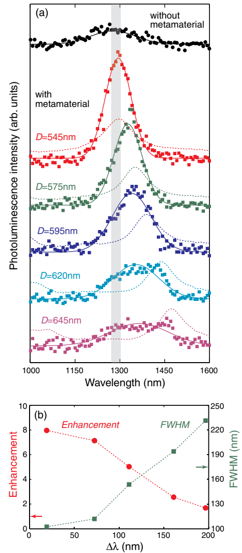
FIG. 2 (color online). Photoluminescence controlled by plasmonic metamaterials. (a) Photoluminescence spectra of the QDs without (top) and with a metamaterial layer accompanied by Gaussian fits (solid lines). Dotted lines indicate metamaterial absorption spectra. (b) Intensity enhancement and FWHM of the QD-metamaterial photoluminescence spectra. Enhancement is normalized to the photoluminescence peak intensity measured without a metamaterial layer. Reference values measured without a metamaterial layer are indicated by arrows.
