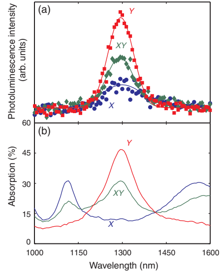
FIG. 3 (color online). Polarization dependence of (a) photoluminescence and (b) absorption, measured for the metamaterial with D = 545 nm. Linear polarizations x and y are introduced in Fig. 1(b), while xy is the intermediate polarization at 45^\circ to x .
