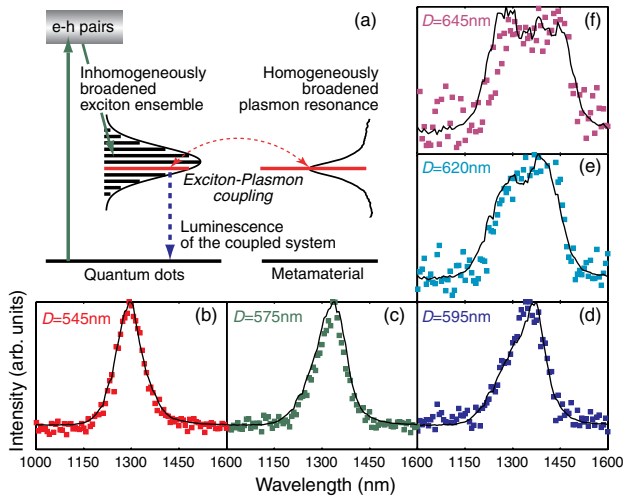
FIG. 4 (color online). Nature of the photoluminescence change in the plasmonic metamaterial. (a) Energy diagram of the QD-metamaterial coupled system. (b–f) Comparison of the measured photoluminescence (data points) with \chi_A(\lambda) = PL_0(\lambda) \times A(\lambda) (lines) for metamaterials with different unit cell sizes ranging from D = 545 nm to 645 nm. Here, PL_0(\lambda) is normal QD photoluminescence without a metamaterial structure, and A(\lambda) is the metamaterial's absorption spectrum.
