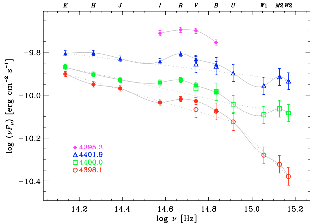
Fig. 5. Spectral energy distributions (SEDs) of 0716+714 in late October 2007, constructed with W2M2W1UBV data from Swift-UVOT (empty symbols) and ground-based GASP-WEBT BVR1JHK data (filled symbols). The numbers in the legend refer to the Julian Dates of the observations. The dotted lines connect the K , U , and W2 data; together with the cubic splines through the spectra, they help to better distinguish the main features of the SEDs (see text).
